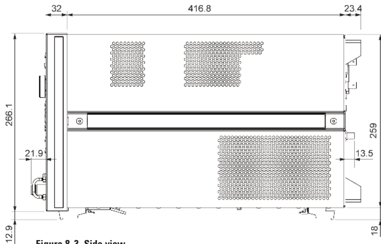
Figure 8-3. Side view
