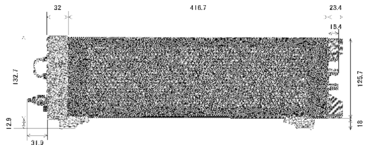
Figure 10-8. Side view
